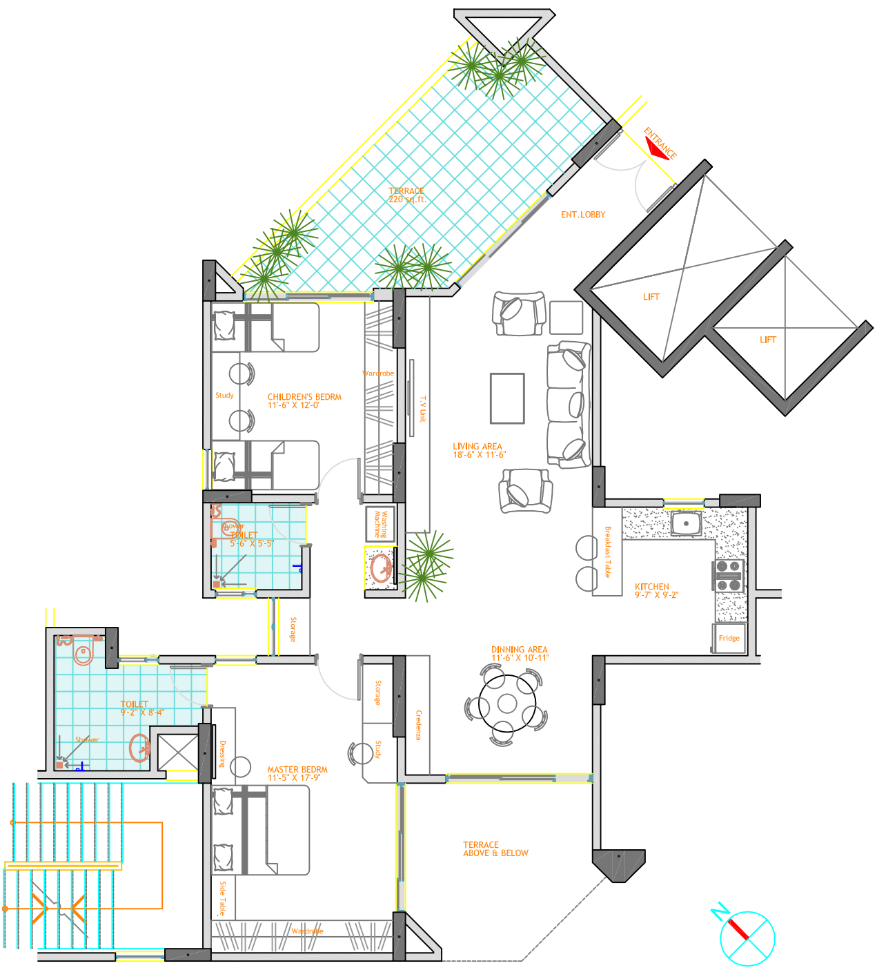
STANDARD LAYOUT FOR SERVICES G- 203,403,603,803,1003,1203
